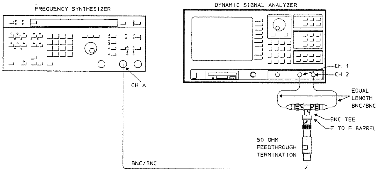
Figure 3-8. Input Coupling Test Setup
