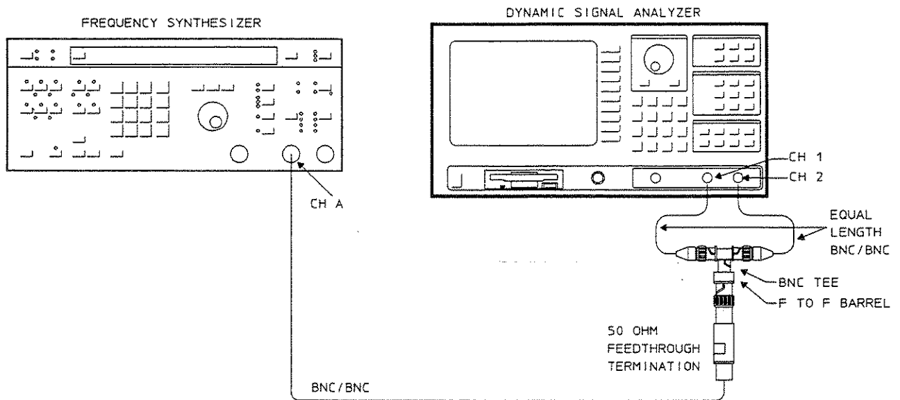
Figure 3-16. Harmonic Distortion Test Setup
